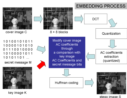
Figure 5: ISC embedding process.
